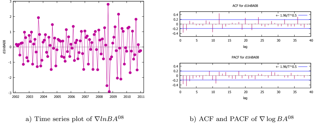
Figure 4: Graph of \nabla \log BA^{08}
